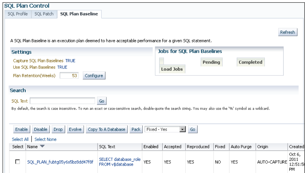
Figure 28-1 SQL Plan Baseline Subpage
