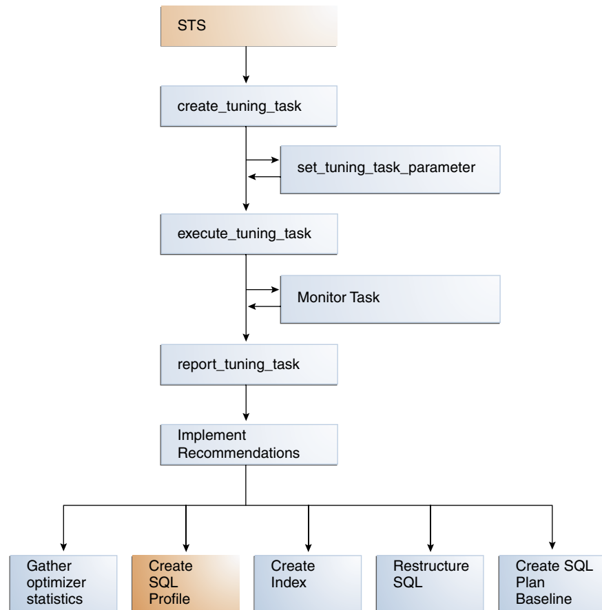
Figure 24-12 SQL Tuning Advisor APIs
