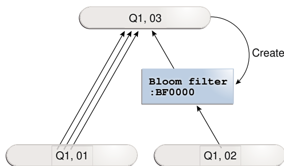
Figure 9-8 Bloom Filter
